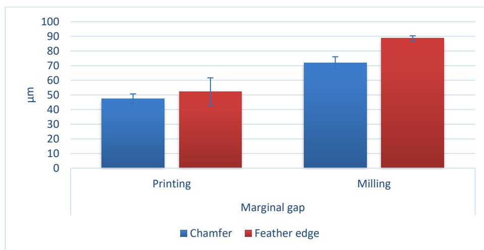
Fig. 6: Bar chart showing mean and standard deviation values of marginal gap (A).
